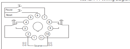
JSS48A-11 Wiring diagram
