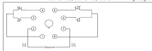
JSS48A-S Wiring diagram
