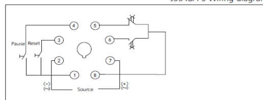
JSS48A-S Wiring diagram
