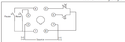
JSS48A-11 Wiring diagram
